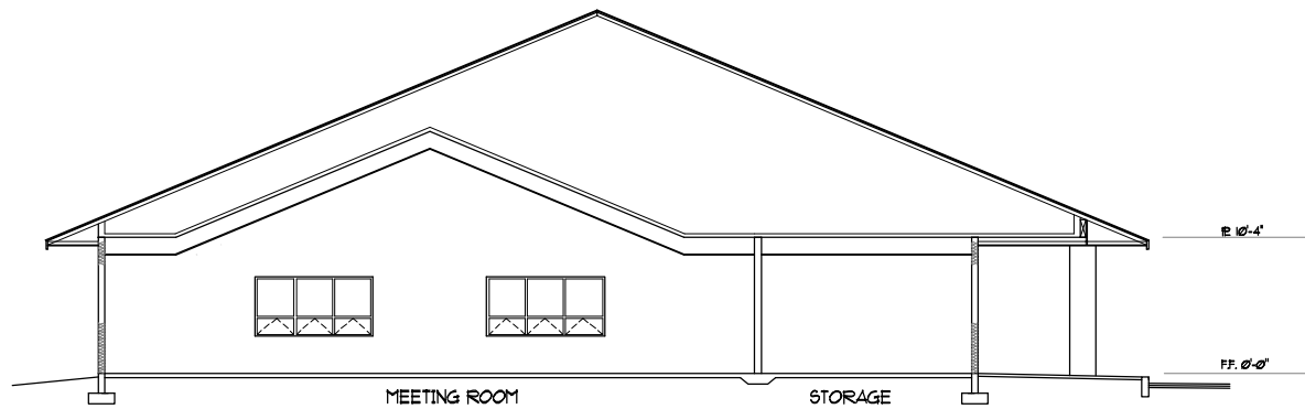
SECTION THRU MULTI-USE WING
