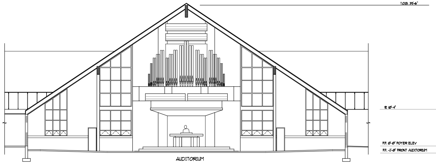
CROSS SECTION THRU AUDITORIUM
